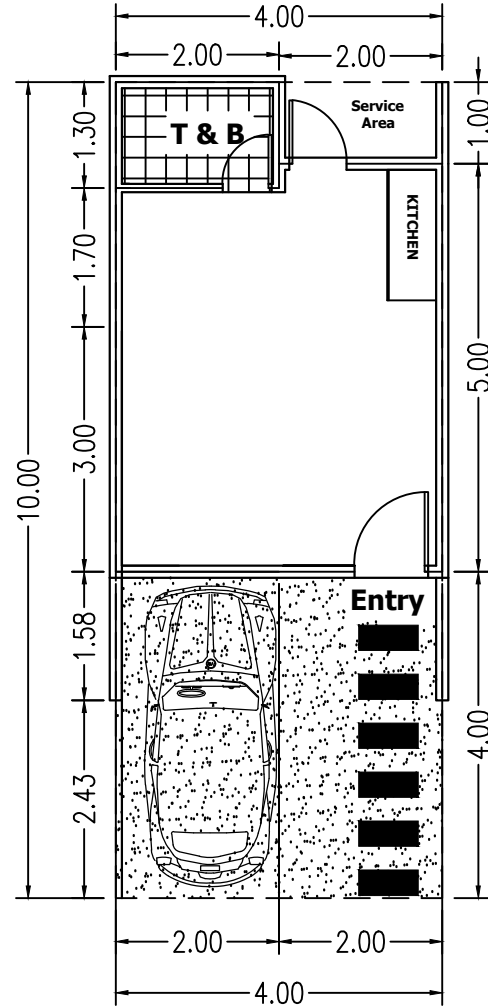
GROUND FLOOR FLOOR AREA= 22.00 sqm
